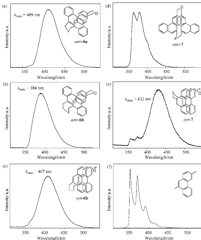
Figure 3. Fluorescence spectra of (a) anti - 6a , (b) anti - 6b , (c) syn - 6b , (d) anti - 7 , (e) syn - 7 , and (f) 3,9-dimethylphenanthrene on 280-nm excitation in cyclohexane at room temperature.
