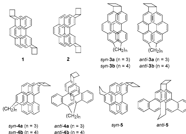
Figure 1. Phenanthrenophanes so far prepared.
