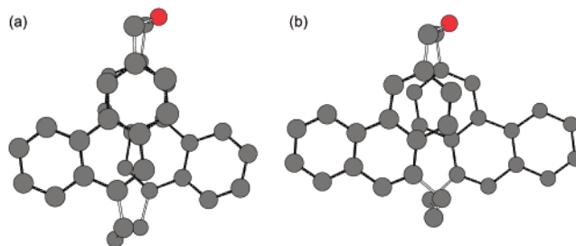
Figure 2. Optimized structures of (a) anti - 6b and (b) anti - 7 determined by MM2 calculations.
